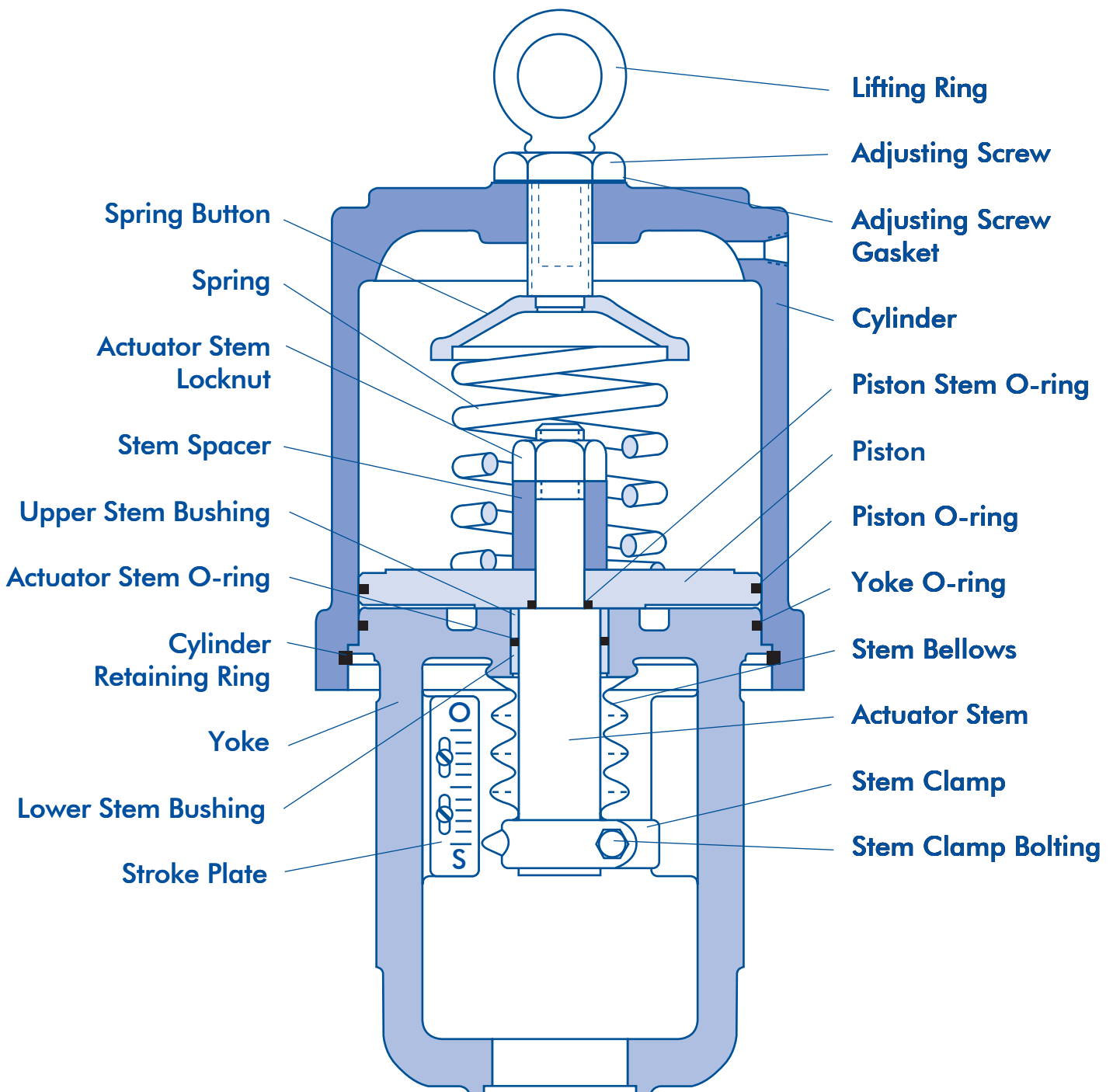
Figure 1: Spring Cylinder Linear Actuator
