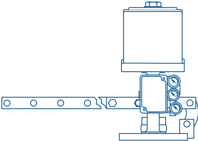
Figure 18: Lever Actuators
