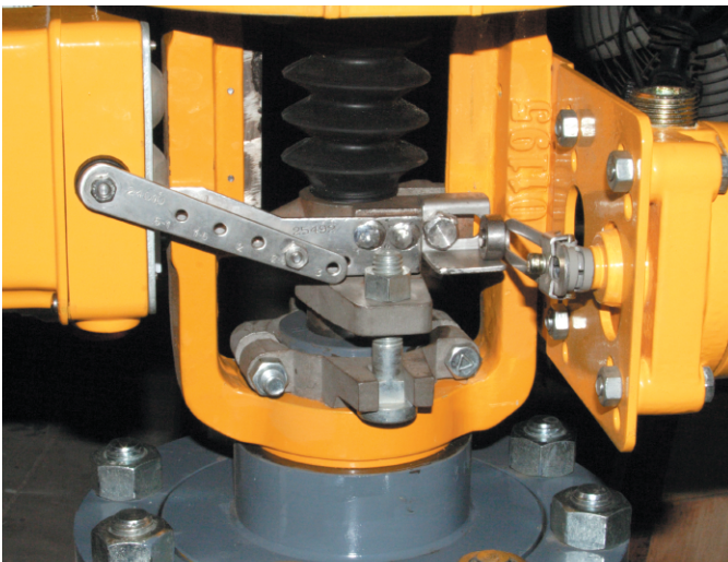
Figure 21: Limit Switches
